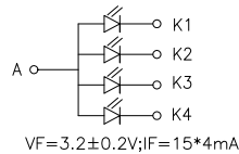
BACKLIGHT CIRCUIT DIAGRAM
